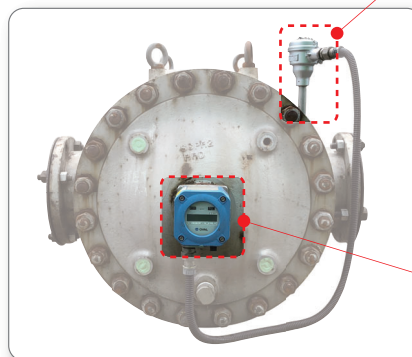
Positive Displacement flowmeter with ULTRA register with automatic temperature compensator
