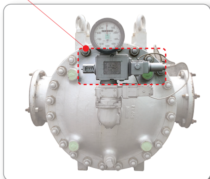
Positive Displacement flowmeter with mechanical automatic temperature compensator
